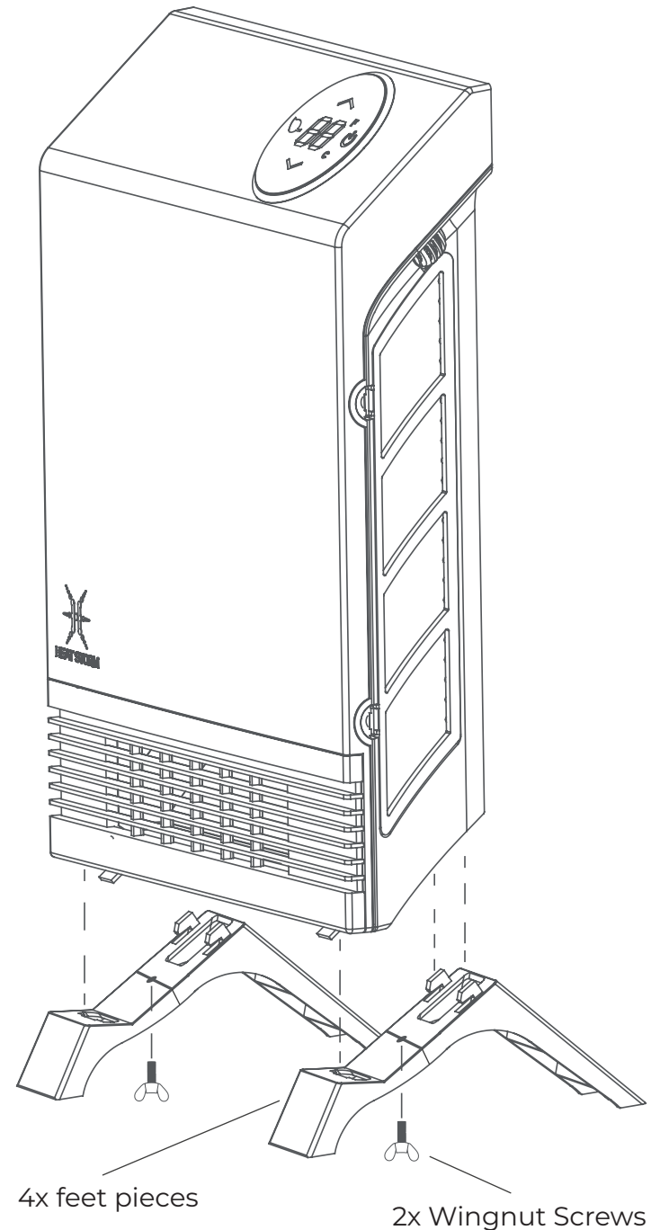
FEET INSTALLATION
